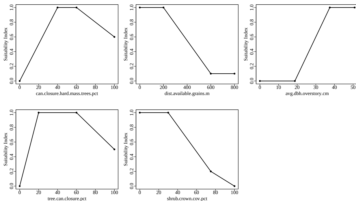
Figure 1. Suitability index graphs for variables included in the foxsquirrel model in ecorest .
