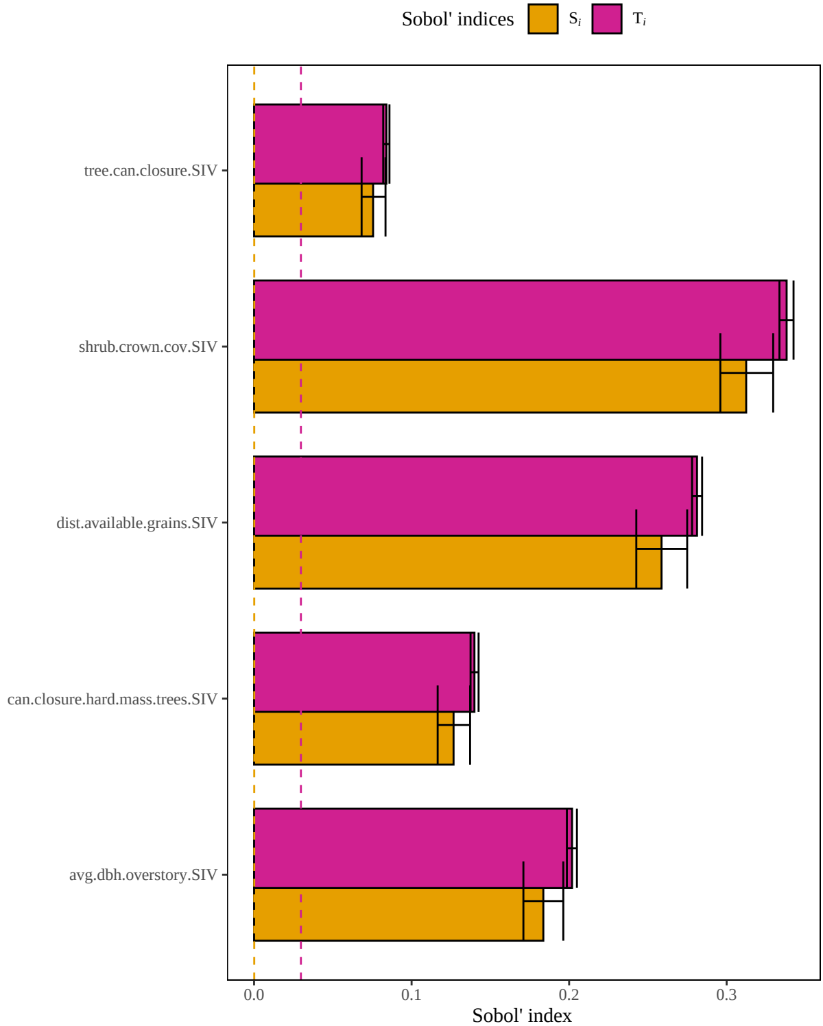
Figure 5. Results of a sensitivity analysis for the foxsqurrel model based on a geometric mean structure. Dashed lines represent baseline numerical approximation error for S_i and T_i ( i.e. , dummy variables).
